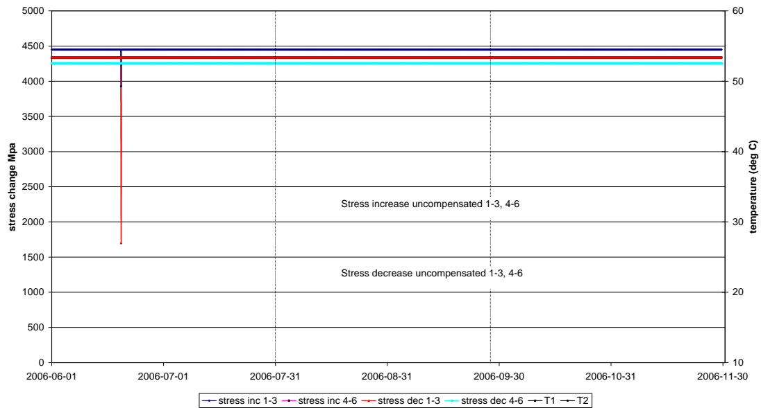
Biaxial stressmeter C6 Maximum stress increase and stress decrease in plane perpendicular to borehole axis
