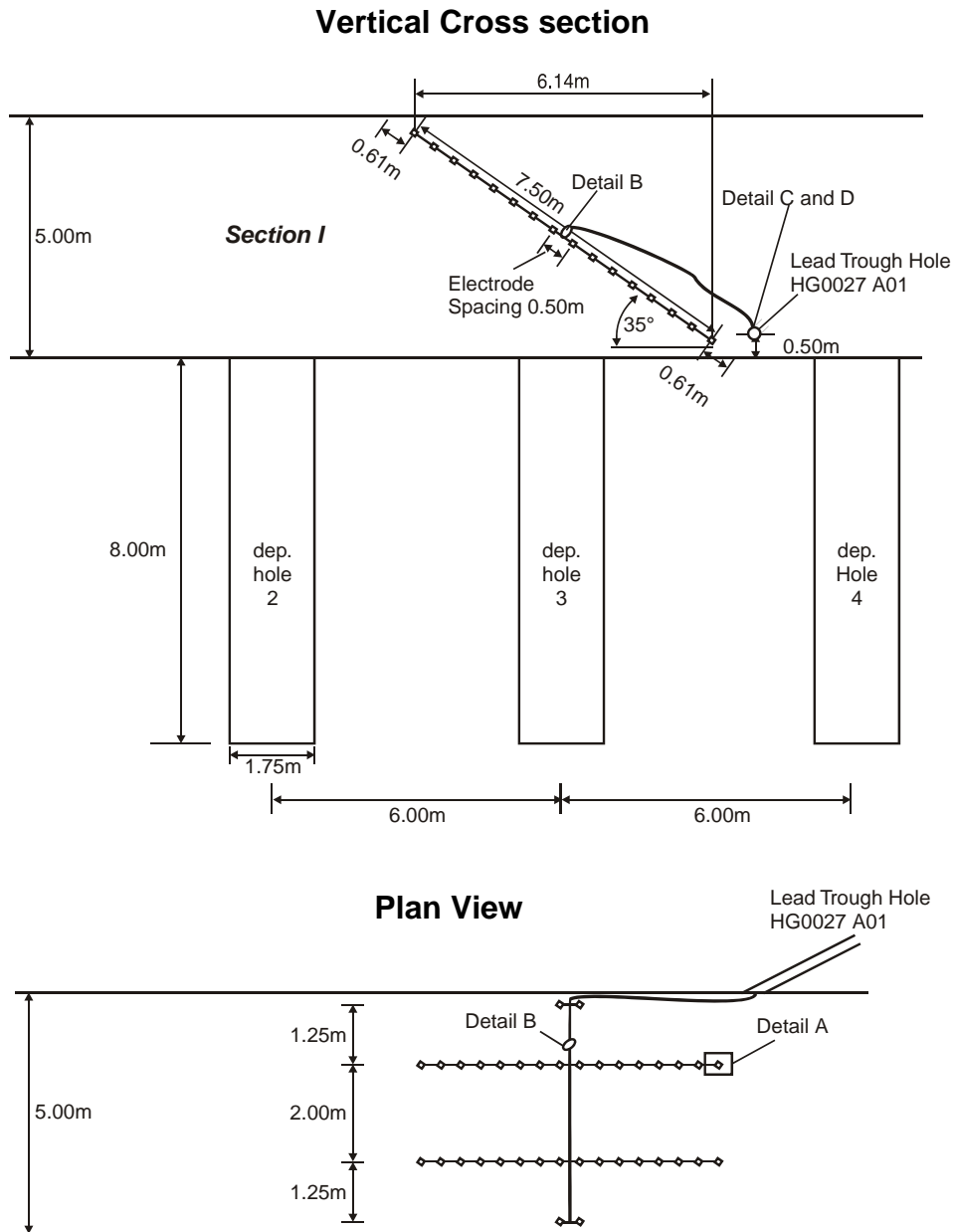
Figure 2-1. Electrode array in the backfill in section 1.
