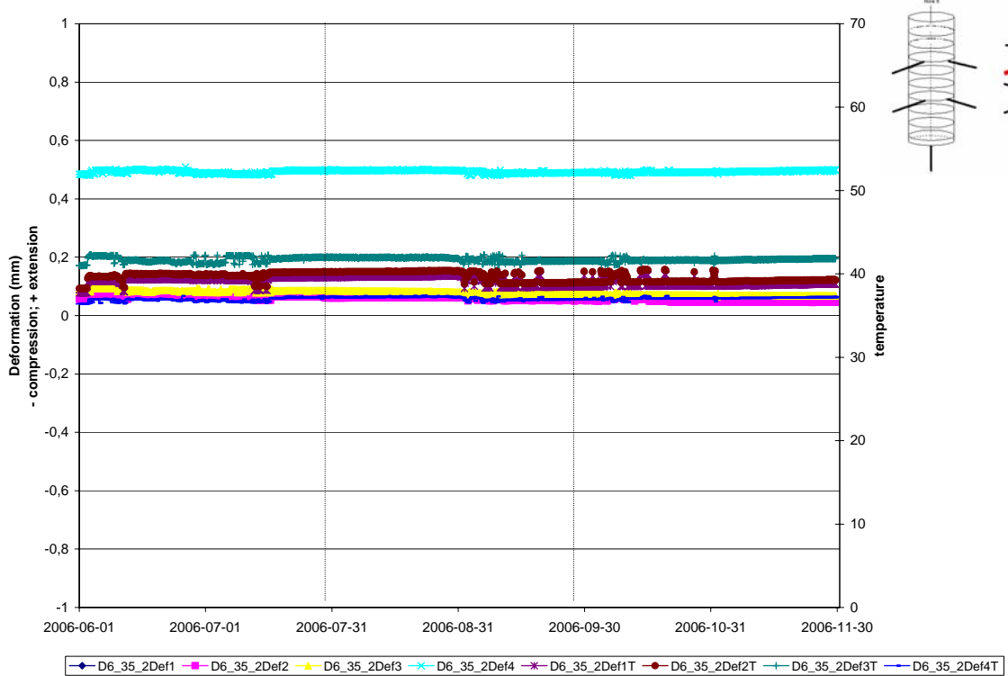
Deformation measurements Borehole D6:3.5(2)
