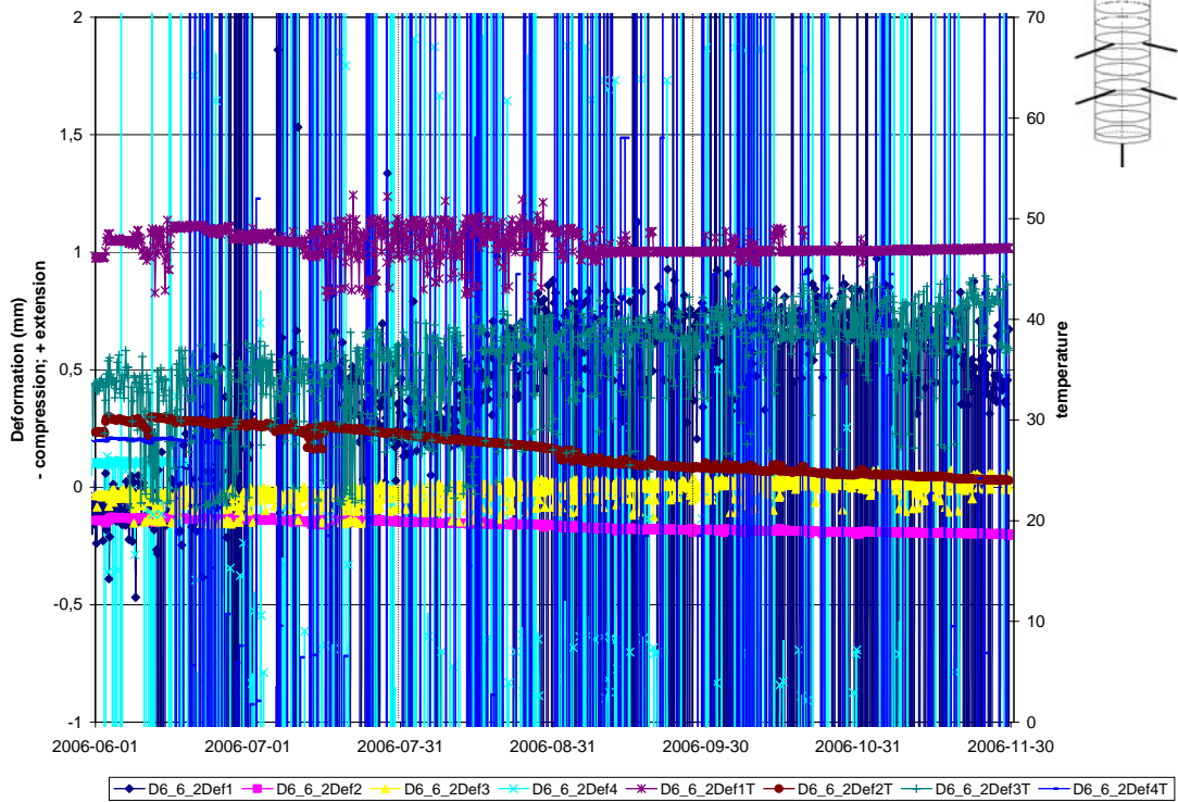
Deformation measurements Borehole D6:6(2)
