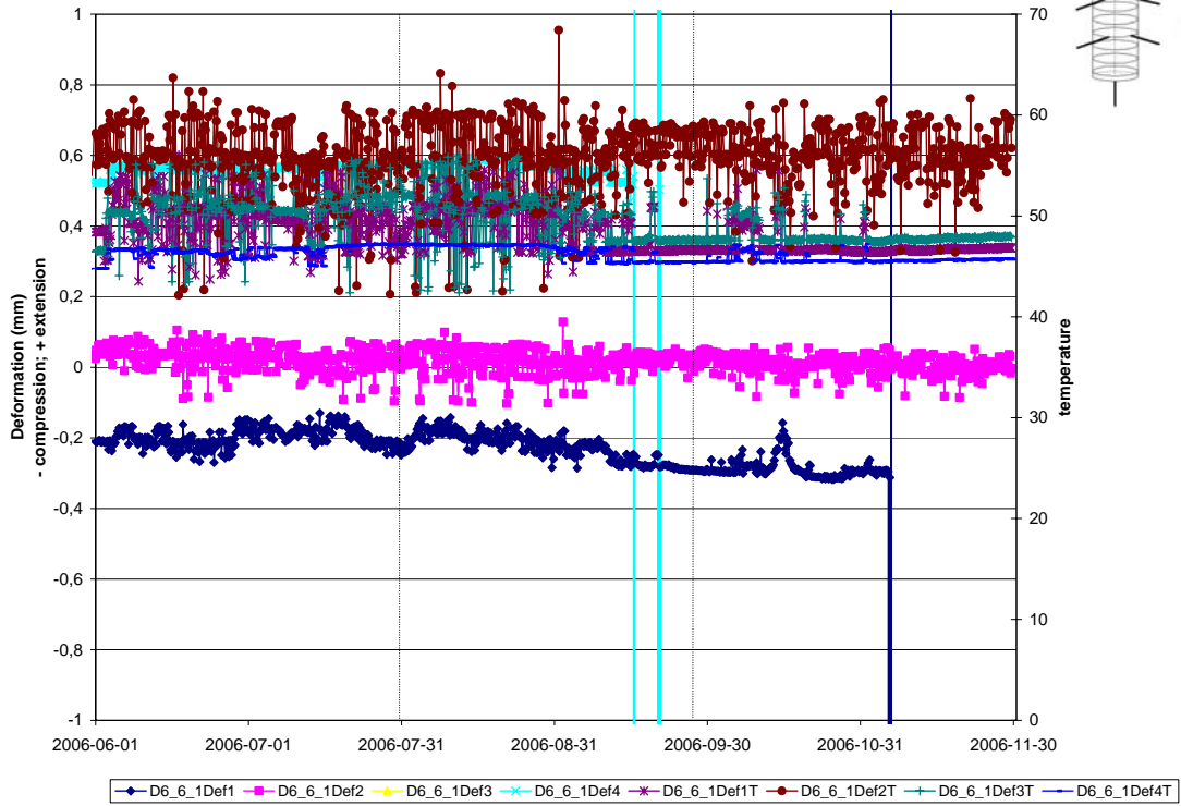
Deformation measurements Borehole D6:6(1)
