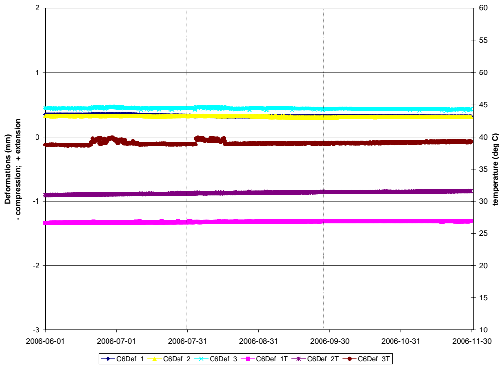
Vertical deformations adjacent to Deposition Hole 6 in borehole C6
