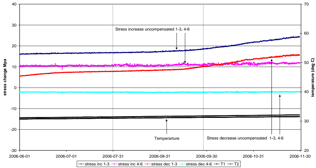
Biaxial stressmeter A6 Maximum stress increase and stress decrease in plane perpendicular to borehole axis
