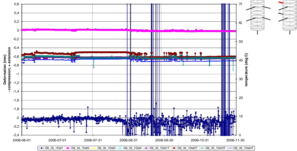
Deformation measurements Borehole D6:3.5(1)
